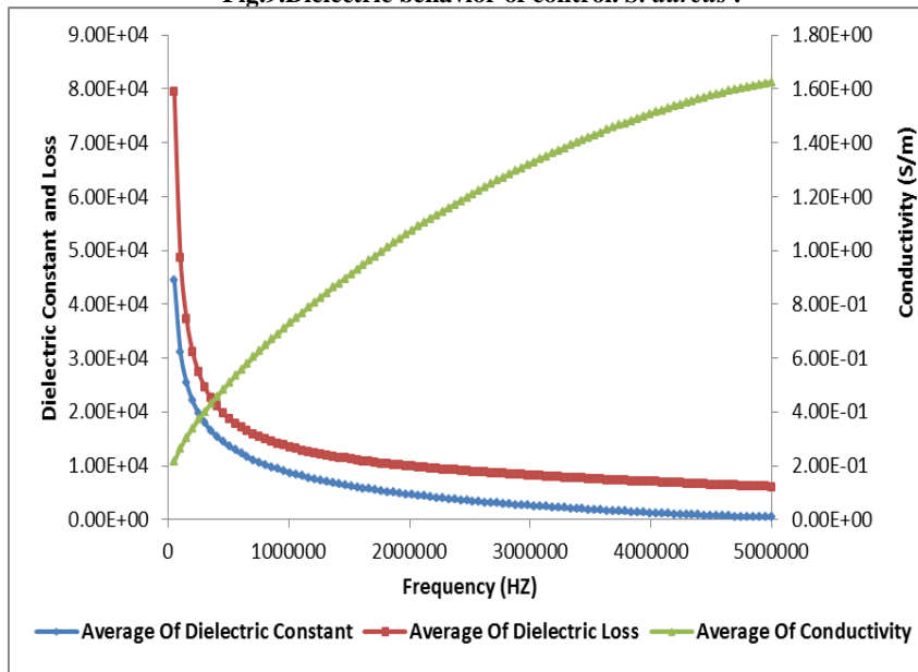
Fig.10. Dielectric behavior of S. aureus treated with Ag-NPs.
