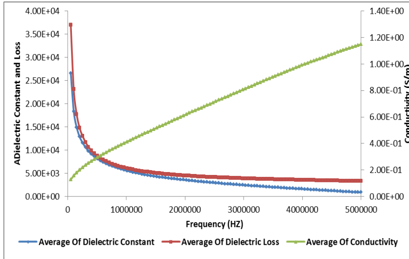
Fig.9. Dielectric behavior of control. S. aureus .
