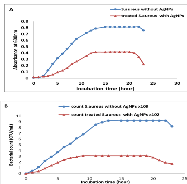
Fig. 1. (A&B). Growth curves of S. aureus cells exposed to Ag-NPs at normal condition.
