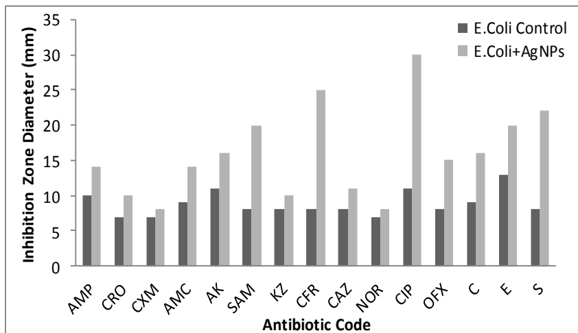
Fig. 8. Histogram for inhibitory zone diameter for unexposed E.coli and treated with Ag-NPs
