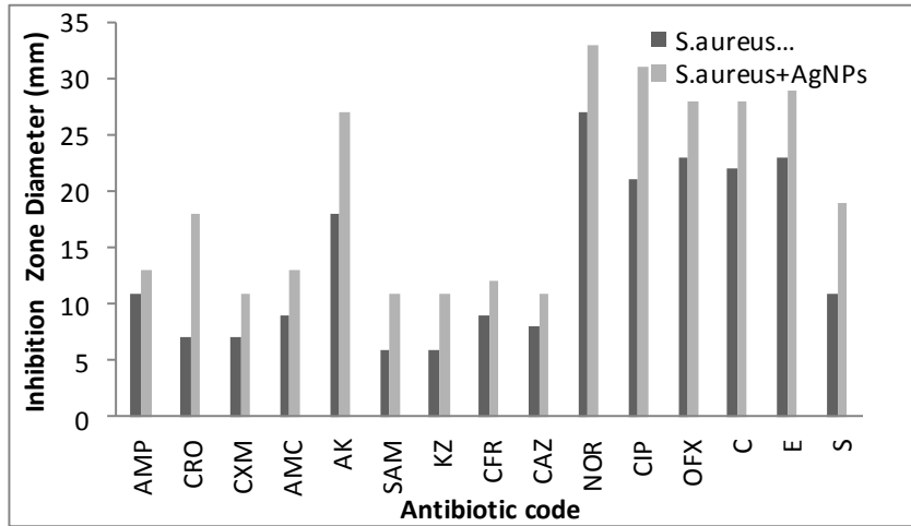
Fig. 7. Histogram for inhibitory zone diameter for unexposed S.aureus and treated with Ag-NPs.
