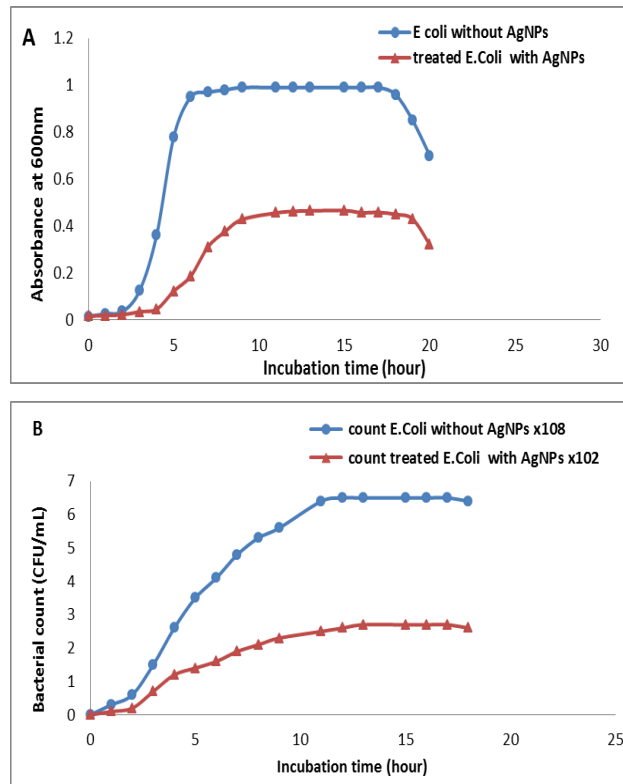
Fig. 2. (A&B). Growth curves of E.Coli cells exposed to Ag-NPs at normal condition.
