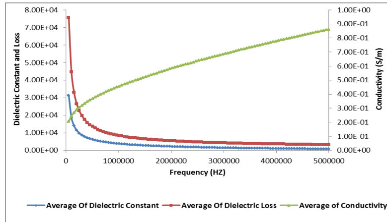
Fig. 11. Dielectric behavior of control. E.Coli .
